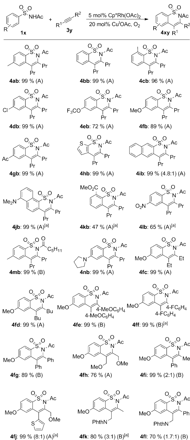
Scheme 2. Scope of the sultam formation. Conditions A:
